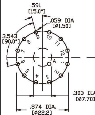
8404-1 MODELS
