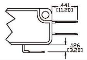
C TYPE (QUICK CONNECT 250 series)
